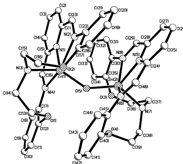
Fig. 3 The molecular structure of the cation from complex 3 ·CH 3 CN, [Zn_2L^2(OH)][ClO_4]_3 \cdot CH_3CN . Selected bonds and angles: Zn(1)–O(5), 1.904(2); Zn(2)–O(5), 1.910(2); Zn(1)–N(3), 2.066(3); Zn(2)–N(5), 2.107(3); Zn(1)–N(1), 2.094(3); Zn(2)–N(7), 2.108(3); Zn(1)–N(2), 2.249(3); Zn(2)–N(8), 2.279(3); Zn(1)–N(4), 2.426(3); Zn(2)–N(6), 2.323(3) Å. O(5)–Zn(1)–N(3), 136.14(11); O(5)–Zn(2)–N(5), 129.92(10); O(5)–Zn(1)–N(1), 121.73(10); O(5)–Zn(2)–N(7), 128.95(10); N(3)–Zn(1)–N(1), 101.24(11); N(5)–Zn(2)–N(7), 101.12(11); O(5)–Zn(1)–N(2), 97.98(10); O(5)–Zn(2)–N(8), 97.81(10); N(3)–Zn(1)–N(2), 101.65(11); N(5)–Zn(2)–N(8), 73.50(11); N(1)–Zn(1)–N(2), 74.77(10); N(7)–Zn(2)–N(8), 97.60(10); O(5)–Zn(1)–N(4), 96.82(9); O(5)–Zn(2)–N(6), 95.19(10); N(3)–Zn(1)–N(4), 87.73(10); N(5)–Zn(2)–N(6), 72.37(11); N(1)–Zn(1)–N(4), 72.06(10); N(7)–Zn(2)–N(6), 99.99(10); N(2)–Zn(1)–N(4), 146.69(10); N(8)–Zn(2)–N(6), 143.95(10); Zn(1)–O(5)–Zn(2), 141.50 (12) o .
